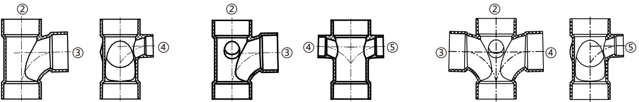
SANITARY TEE W/ LEFT SIDE INLET SANITARY TEE W/ R & L SIDE INLETS DOUBLE SANITARY TEE, W/SIDE INLET
